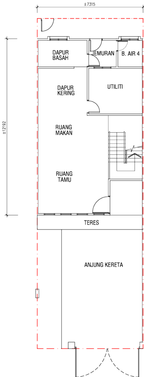
GROUND FLOOR PLAN TERRACE - INTERMEDIATE UNIT (TYPE RT3A) APPLICABLE FOR PLOT: PT 29180
