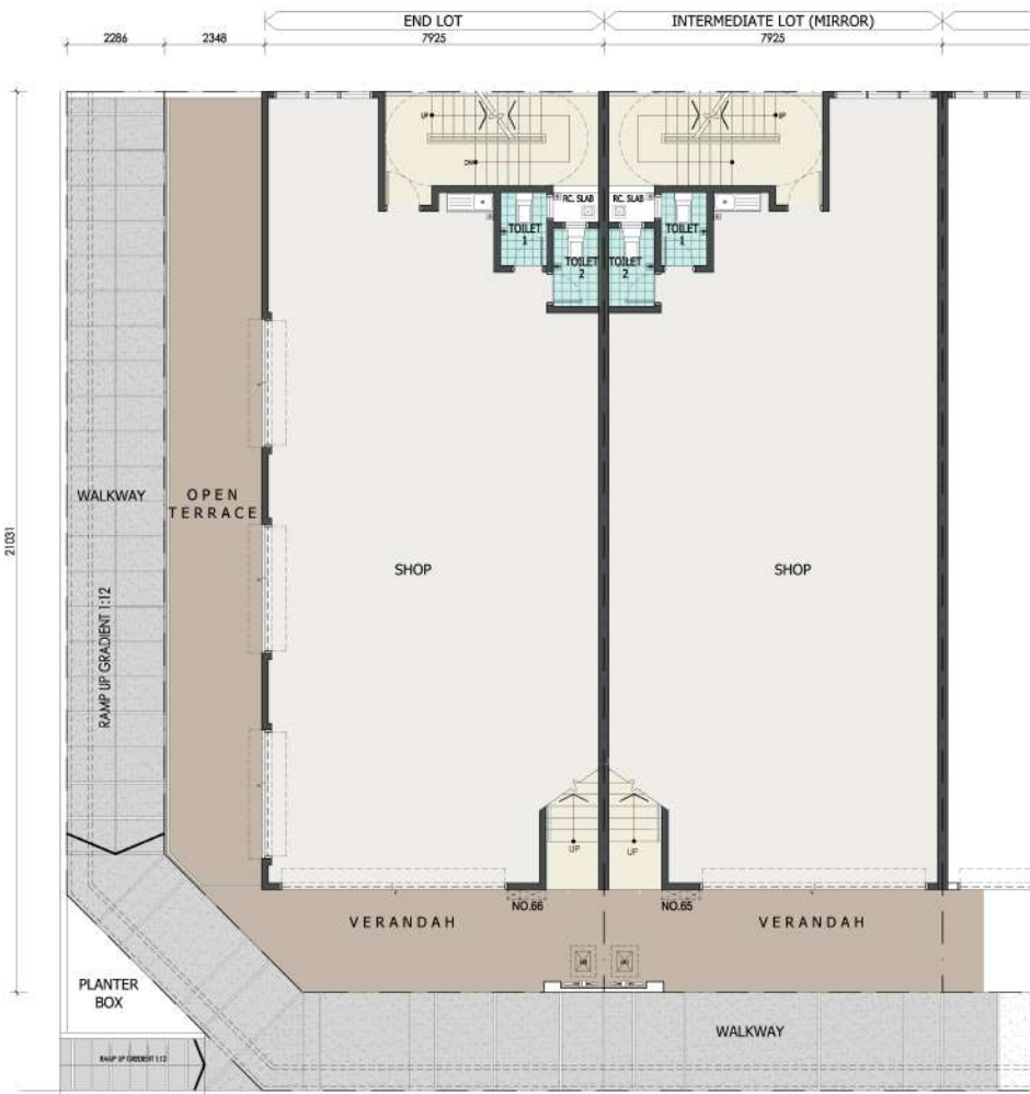
GROUND FLOOR TYPE B-BLOCK 3
