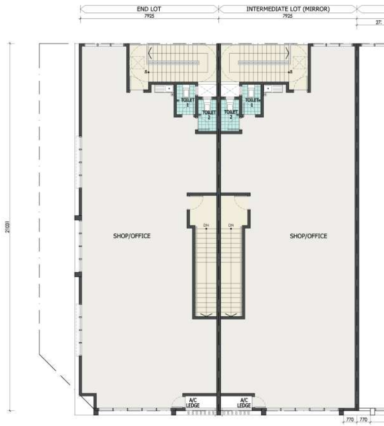
1ST FLOOR PLAN TYPE B- BLOCK 3
