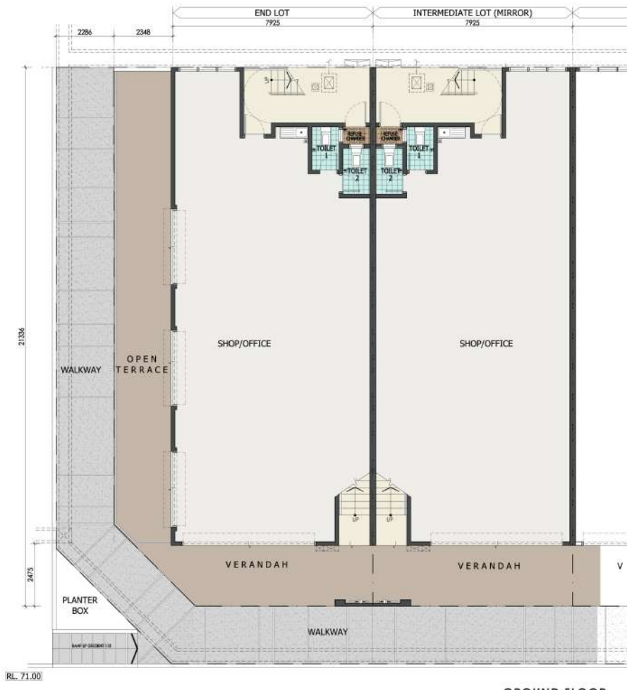
GROUND FLOOR TYPE A- BLOCK 1 & 2
