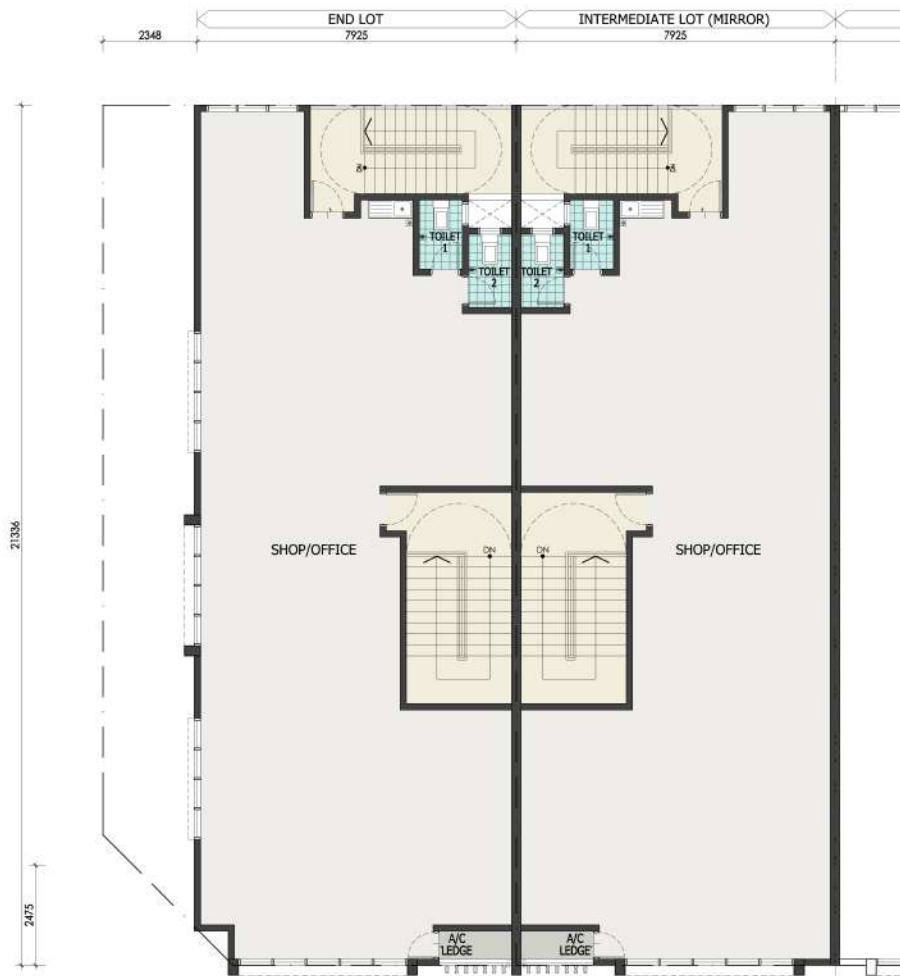
2ND FLOOR PLAN TYPE A- BLOCK 1 & 2
