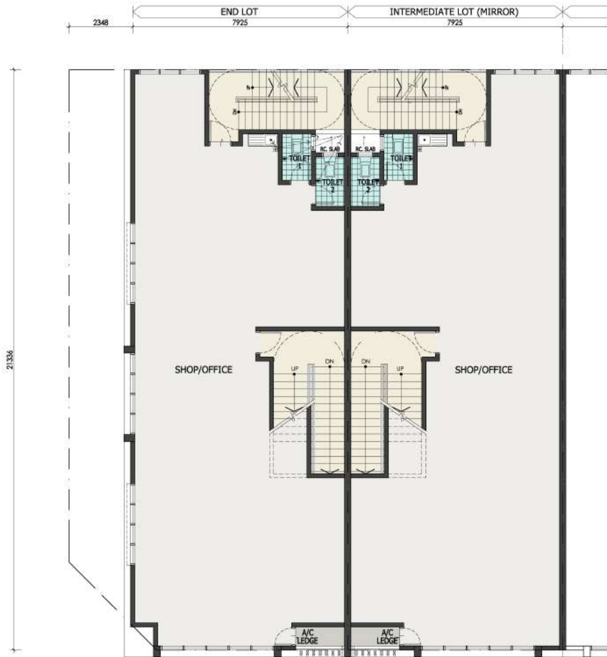
1ST FLOOR PLAN TYPE A-BLOCK 1 & 2
