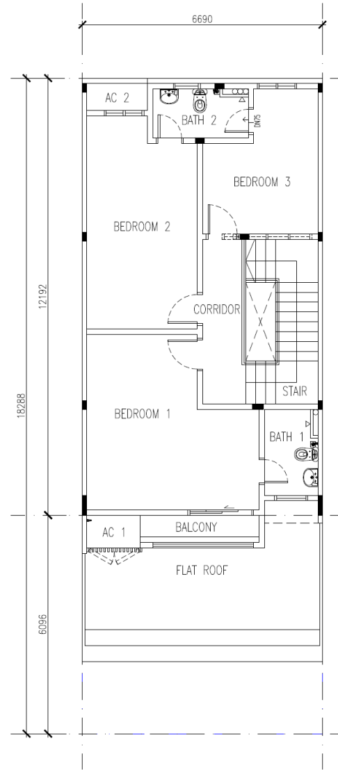
TYPE C - FIRST FLOOR PLAN INTERMEDIATE UNIT
