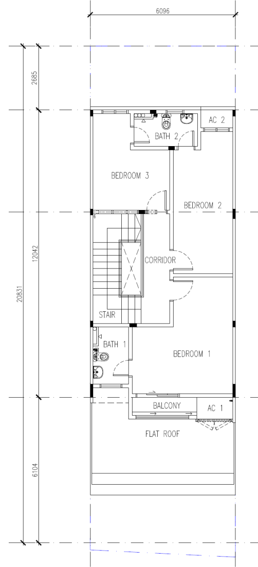
TYPE E - FIRST FLOOR PLAN INTERMEDIATE UNIT
