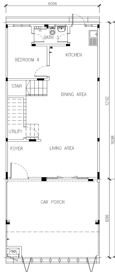
TYPE A - GROUND FLOOR PLAN INTERMEDIATE UNIT
