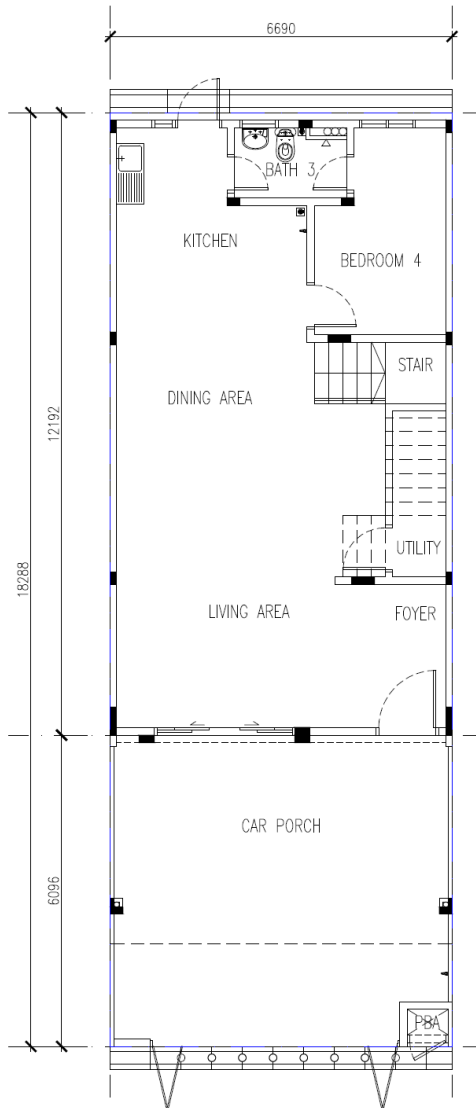
TYPE C - GROUND FLOOR PLAN INTERMEDIATE UNIT
