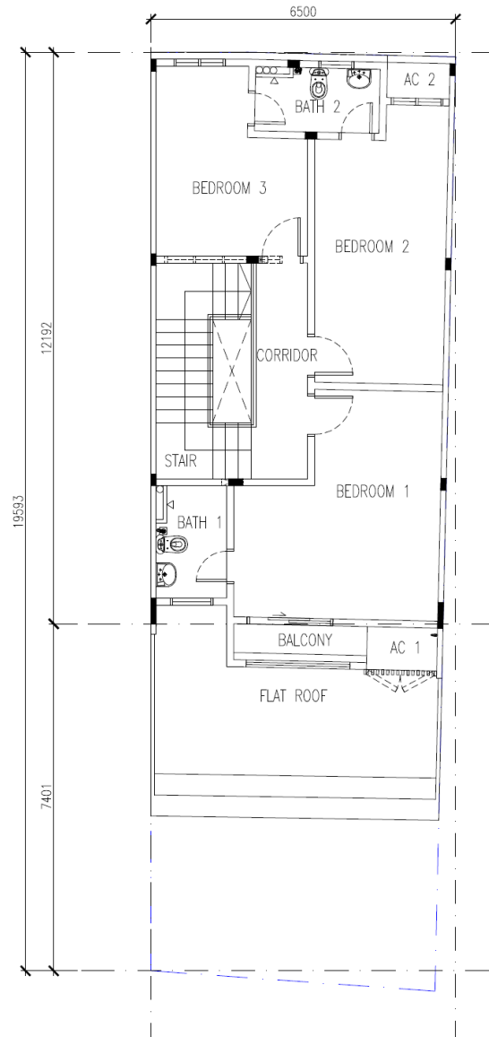
TYPE D - FIRST FLOOR PLAN INTERMEDIATE UNIT
