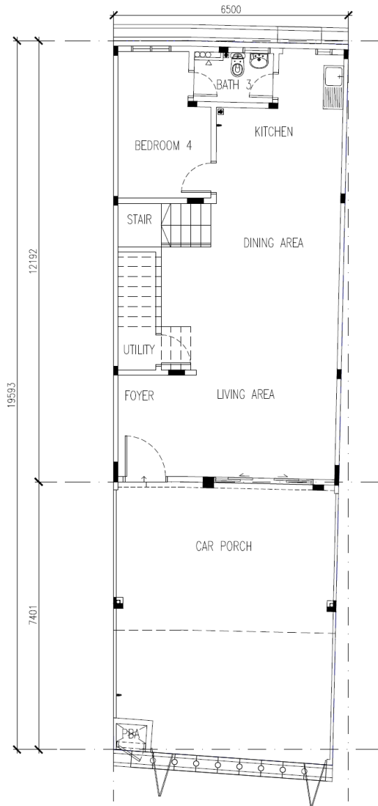
TYPE D - GROUND FLOOR PLAN INTERMEDIATE UNIT
