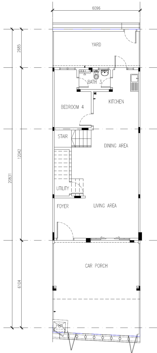
TYPE E - GROUND FLOOR PLAN INTERMEDIATE UNIT
